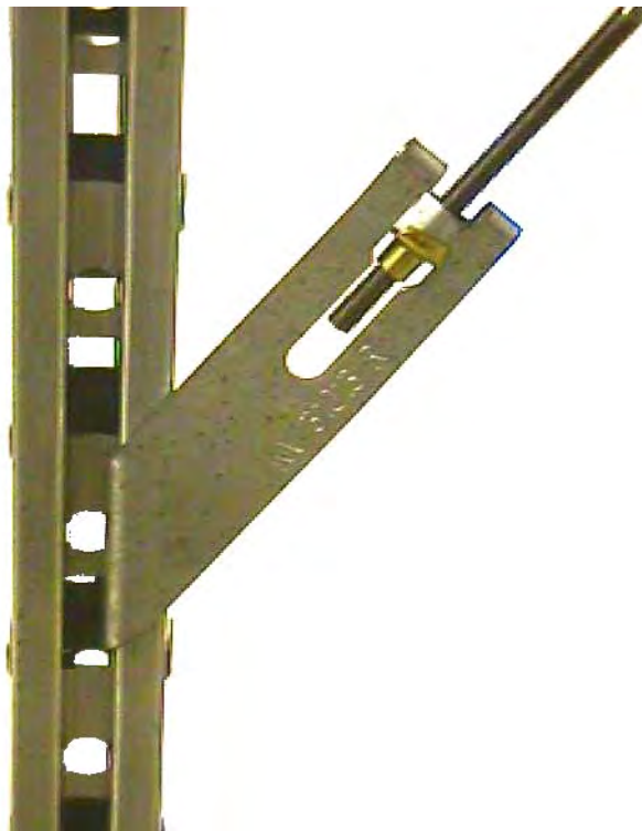
Rear of post showing typical cross-brace connection
